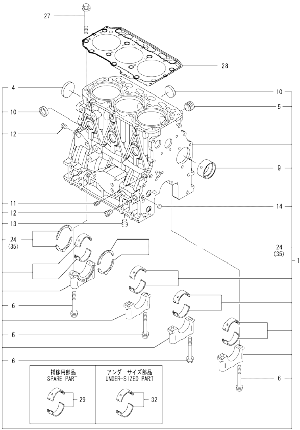
0CW10-M47200 3TNV84T-BGKM Fig.1. CYLINDER BLOCK
